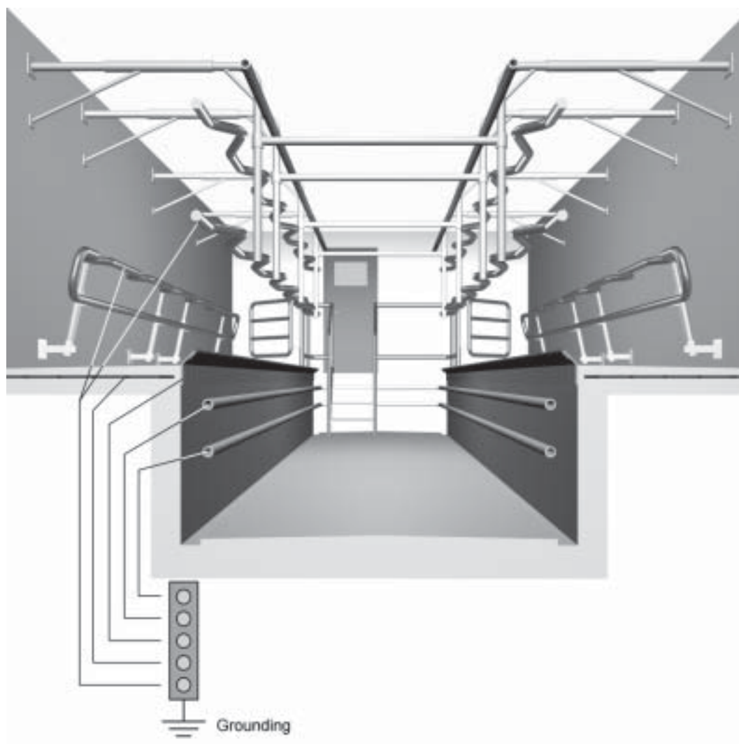
Figure 6.6 Example of equipment potential bonding in milking parlour.
